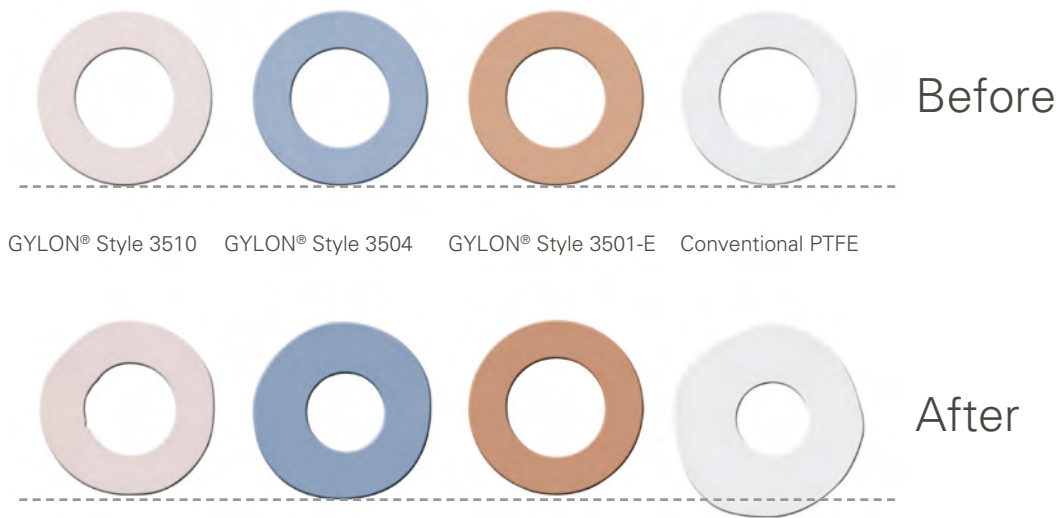
A comparison between GYLON® flat gaskets and un-filled PTFE after exposure to a load of 14 MPa for one hour at a temperature of 260 °C.
